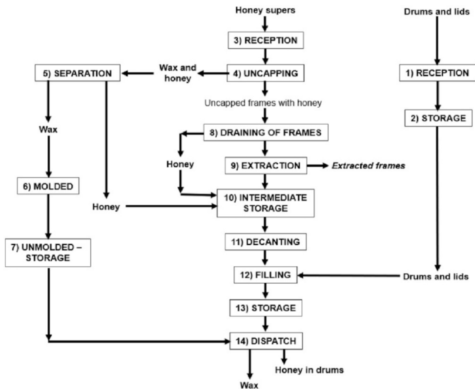
Figure 1. Flow diagram of the honey extraction process [10].
