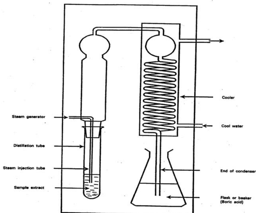
TVB-N steam distillation apparatus
