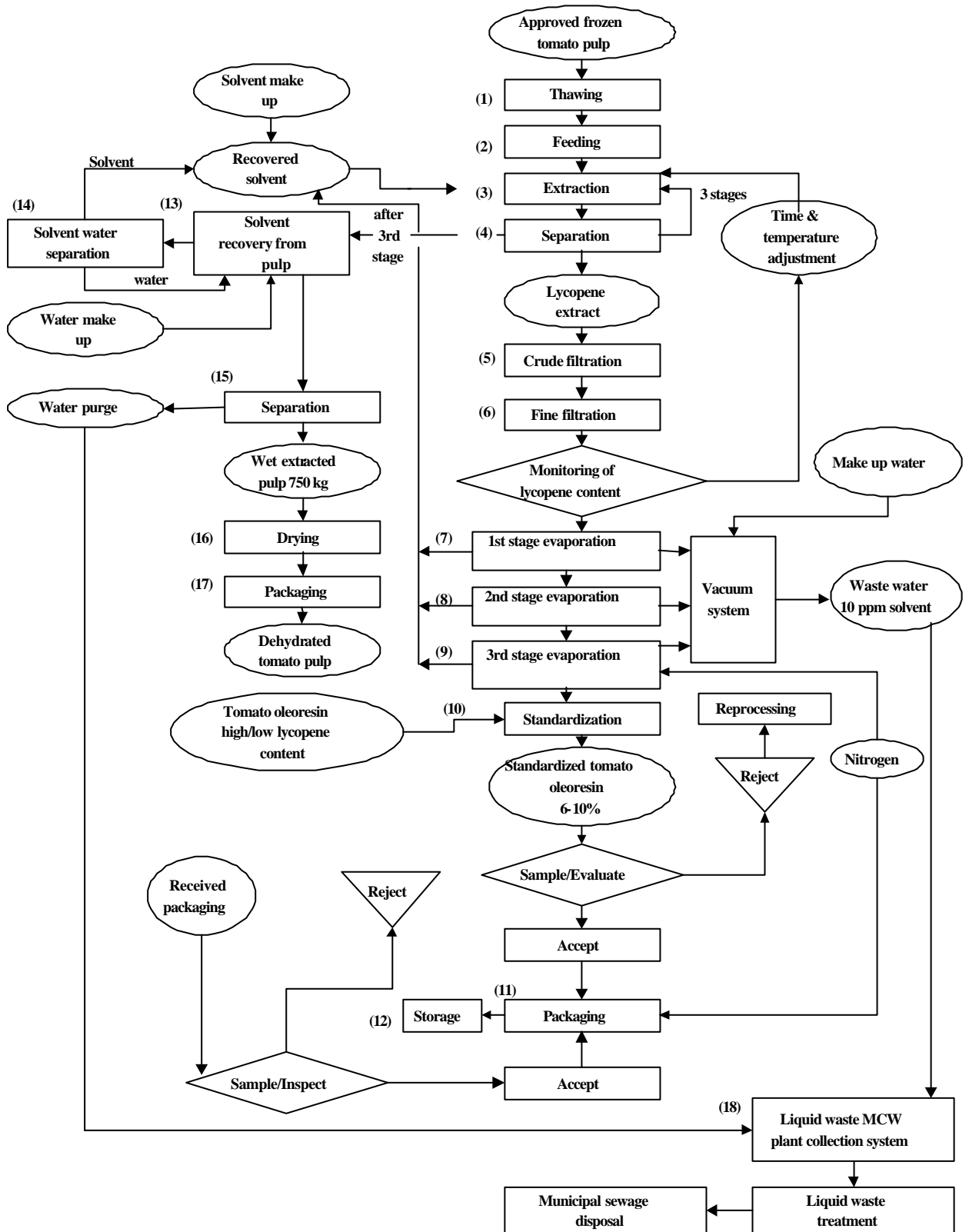
Figure 2. Lyc-O-Mato® Oleoresin 6% production scheme
